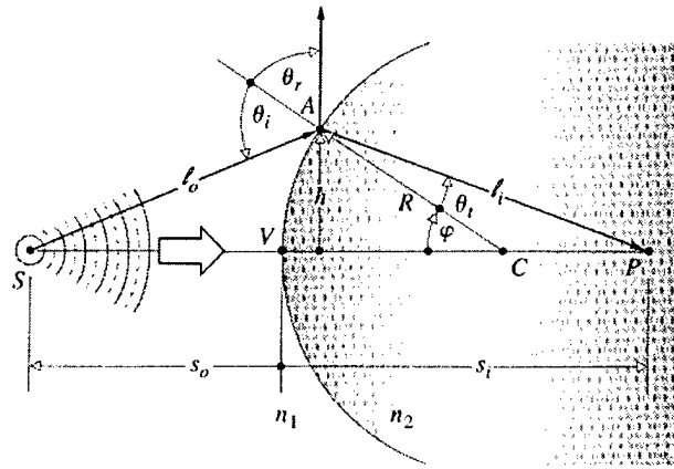
Figure 3.8 Spherical Refraction (21)
